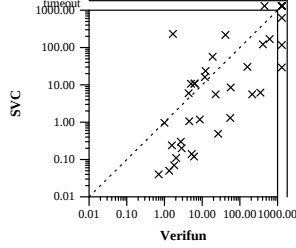
(c) Verifun vs SVC on UCLID and Velev
